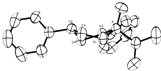
Figure 2. ORTEP plot of (PhC 3 H 5 ONPh)(Me 2 N)PO ( 5 ) showing the twist-boat conformation of the phosphorus-containing six-membered ring.
