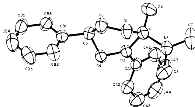
Figure 1. ORTEP plot of (PhC 3 H 5 ONPh)(Me 2 N)PO ( 5 ), with thermal ellipsoids at the 50% probability level. Hydrogen atoms have been omitted for purposes of clarity.
